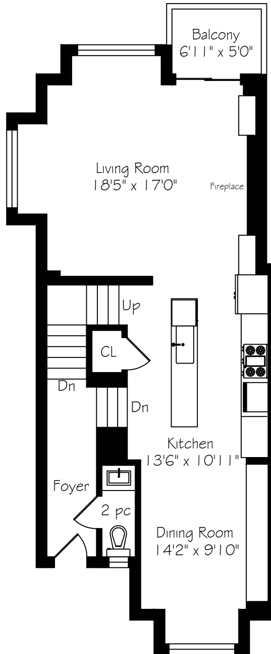
Main / Second Floor 785 Square Feet
